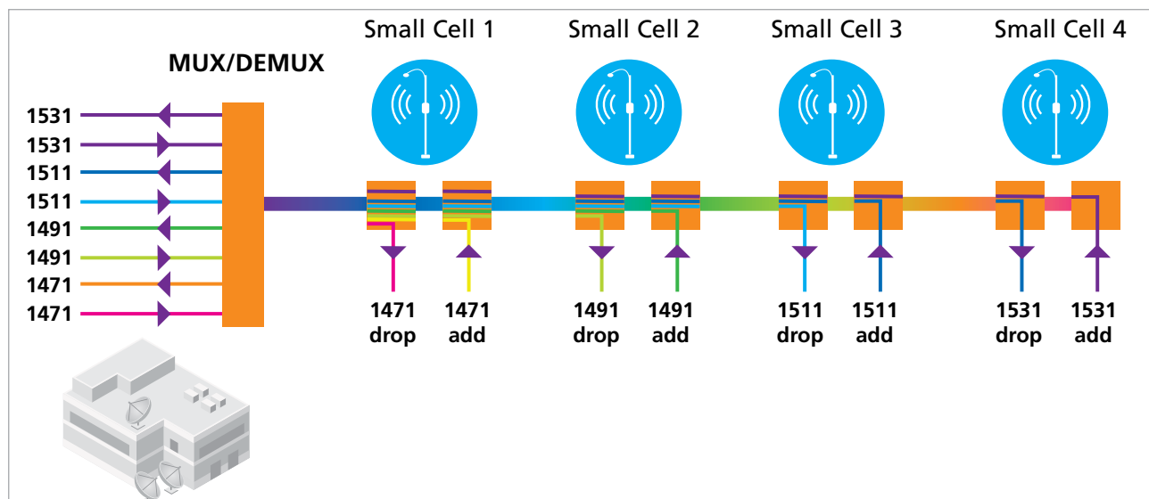
Figure 11: Cell site connectivity with optical add/drop modules
